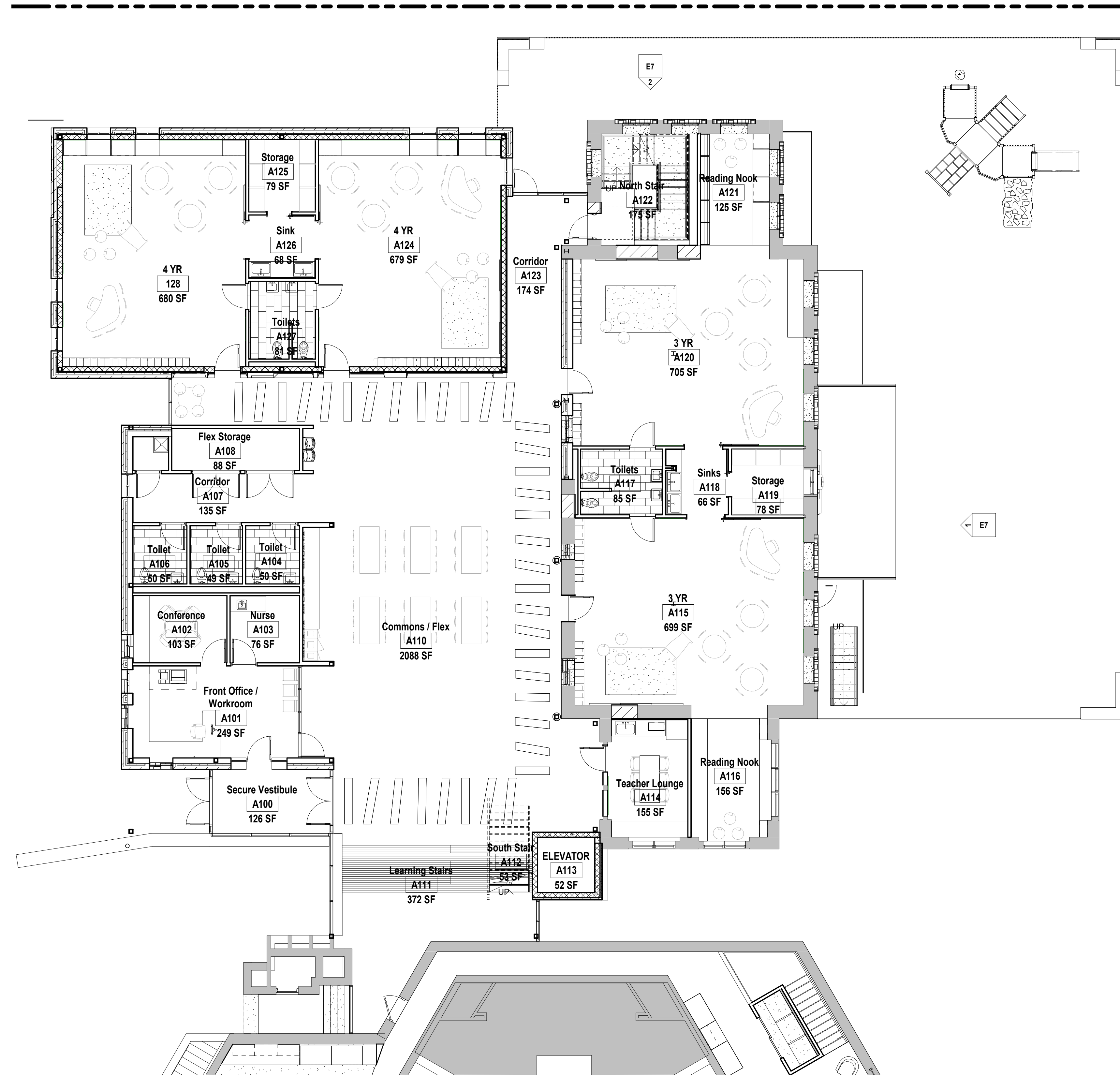
1 Scale ECC - Level 01 1/8" = 1'-0"
